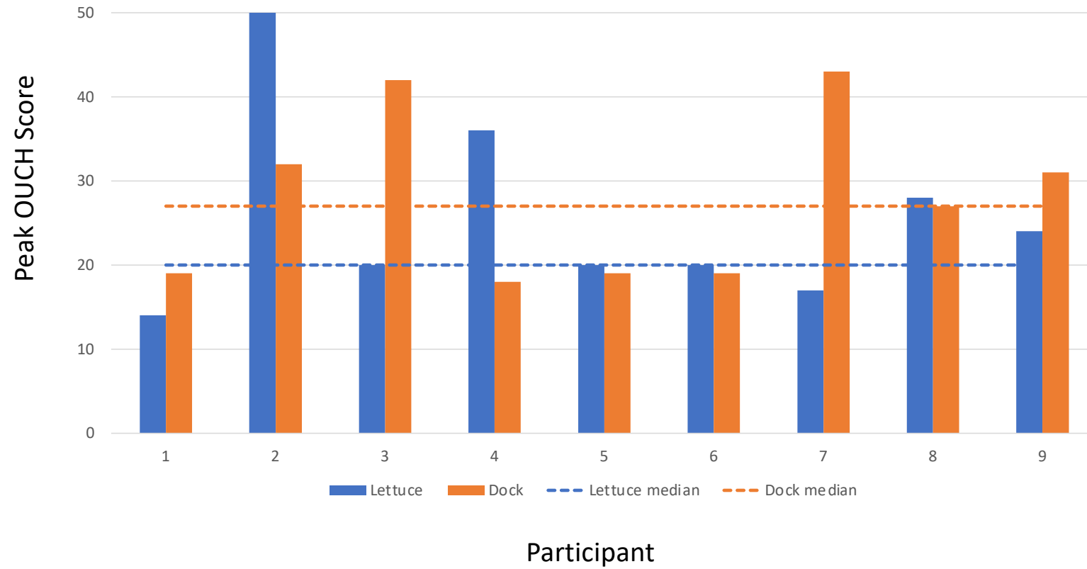
Supplemental Figure 2. Peak OUCH scores in dock and lettuce arms (2-tailed Paired Sign Test, p=0.739 )
