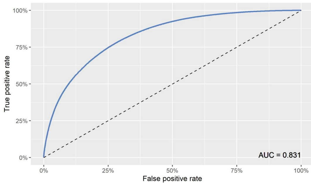
Figure 5: Receiver Operating Characteristic Curve – Logistic general additive model
